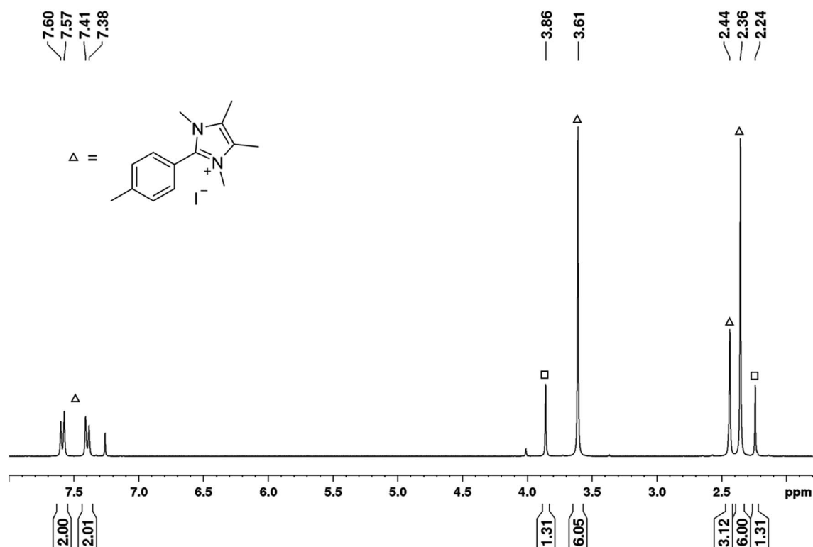
Fig. 7 1 H NMR spectrum recorded in CDCl 3 (400 MHz) of the residue formed in the reaction of stoichiometric amounts of the free NHC with 4-iodotoluene 4I showing the imidazolium salt [\text{4-CH}_3\text{-C}_6\text{H}_4\text{-Me}_2\text{Im}^{\text{Me}}]^+\text{I}^- 8 , and an unknown compound (square).
