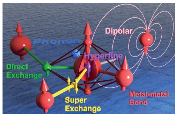
Fig. 1 The schematic model of a Single-Ion Magnet building block (central red sphere) that is coupled to an intra-atomic nuclear spin through the hyperfine interactions (purple), to a radical-bridged spin centre through the direct exchange (green), to a nearby metal ion through a metal–metal bond (red), to a ligand-bridged spin centre through superexchange (yellow), to the dipolar field generated by a distant spin centre (pink), and to the lattice vibration/phonon (the blue ocean).
