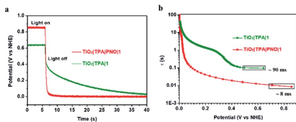
Fig. 9 (a) Open-circuit voltage decays for the electrodes TiO 2 -[TPA|PNO]1 (red) and TiO 2 |[TPA]1 electrodes (green). (b) Electron lifetime derived from eqn (7) plotted as a function of V_{oc} at the transient when illumination (>400 nm, 100 mW cm -2 ) was removed. The results were obtained in 0.1 M phosphate buffer at pH 7.
