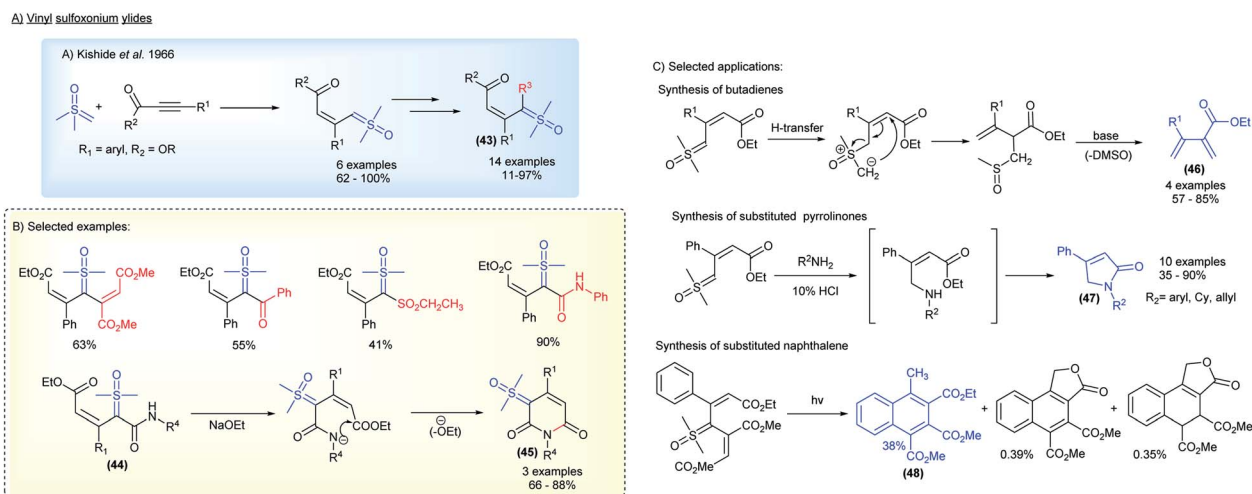
Scheme 7 The synthesis and applications of vinyl sulfoxonium ylides.
