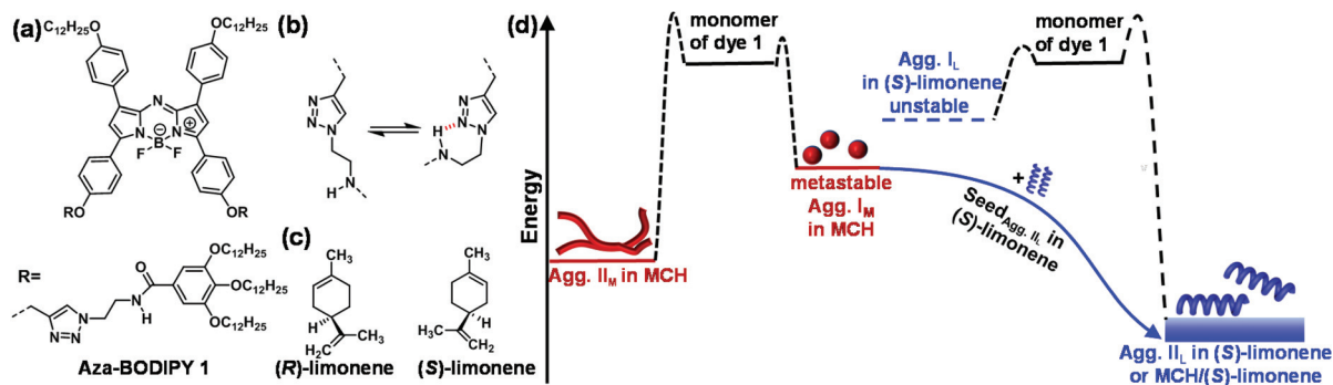
Scheme 1 (a) Chemical structure of aza-BODIPY dye 1 . (b) Conformational interconversion of the intermolecular and intramolecular H-bond moieties in dye 1 . (c) Chemical structures of ( S )- and ( R )-limonene solvents. (d) Schematic illustration of the kinetic aggregation pathways of dye 1 in MCH (left) and ( S )-limonene (right) for the unstable Agg. I L and thermodynamically stable in chiral solvents and the metastable Agg. I M in MCH can be transformed into the chiral Agg. II L via seeded living supramolecular polymerization by adding the seed of Agg. II L in ( S )-limonene.
