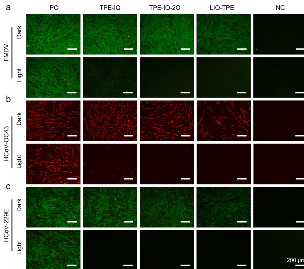
Fig. 4 (a and b) Immunofluorescence studies of (a) BHK-21 cells infected with the FMDV and (b and c) MRC-5 cells infected with (b) HCoV-OC43 and (c) HCoV-229E, which were pre-treated with 5 \mu\text{M} TPE-IQ, TPE-IQ-20 or LIQ-TPE and then subjected to irradiation with white light or storage in the dark for 20 min. PC: the host cells were infected with the untreated virus. NC: the host cells were not infected with the virus. Green channel: \lambda_{\text{ex}} : 460–490 nm, \lambda_{\text{em}} : 520–750 nm; red channel: \lambda_{\text{ex}} : 510–550 nm, \lambda_{\text{em}} : 570–750 nm. Scale bar: 200 \mu\text{m} .
