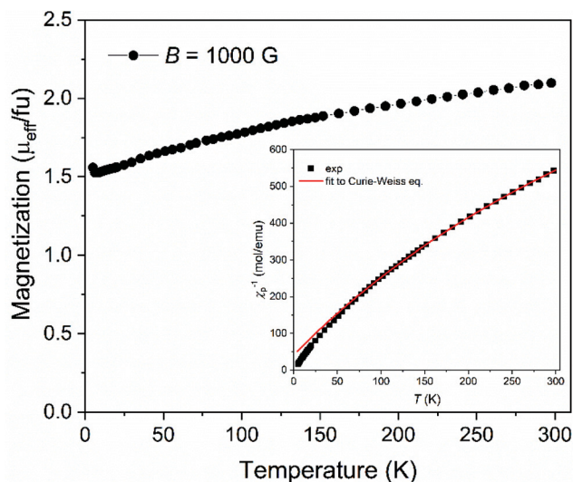
Fig. 1 Magnetic properties of Na[ o - 57 FESAN] powder sample: temperature dependence of the magnetization under a magnetic field of 0.1 T. Inset: temperature dependence of the inverse of the magnetic susceptibility. The solid red line is the fit to the Curie–Weiss law of the experimental data (solid square symbols).
