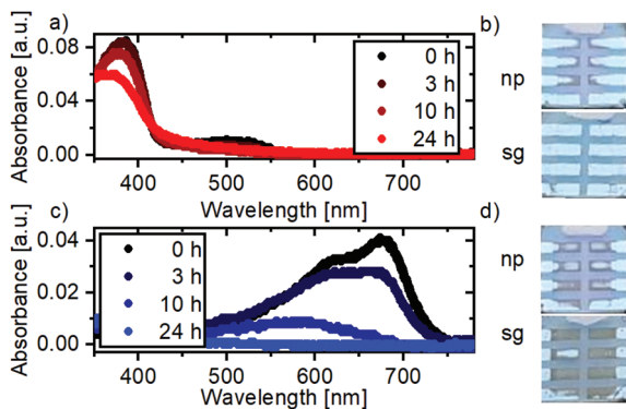
Fig. 6 Dry air and sunlight degradation of the HTL. (a) Absorption changes of a PTAA:C 60 F 48 film. (b) Picture of the electrode of a device using PTAA:C 60 F 48 after 42 h of degradation with either ZnO nano-particle or sol-gel as ETL. (c) Absorption changes in PTB7. (d) Pictures of solar cell electrodes employing PTB7 as HTL and either nano-particle or sol-gel ZnO as ETL.
