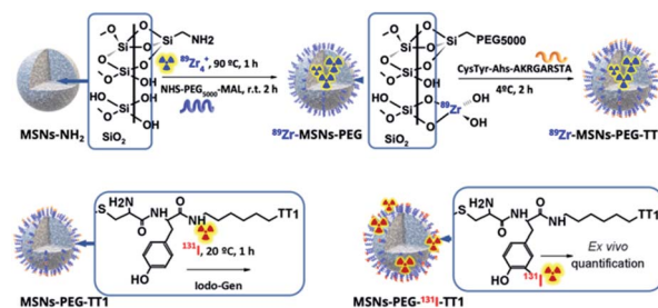
Scheme 1 Strategies for labelling MSNs core with ^{89}\text{Zr} to perform PET imaging studies and tyrosine residue iodination with ^{125}\text{I} in attached peptides to perform ex vivo gamma counting studies.
