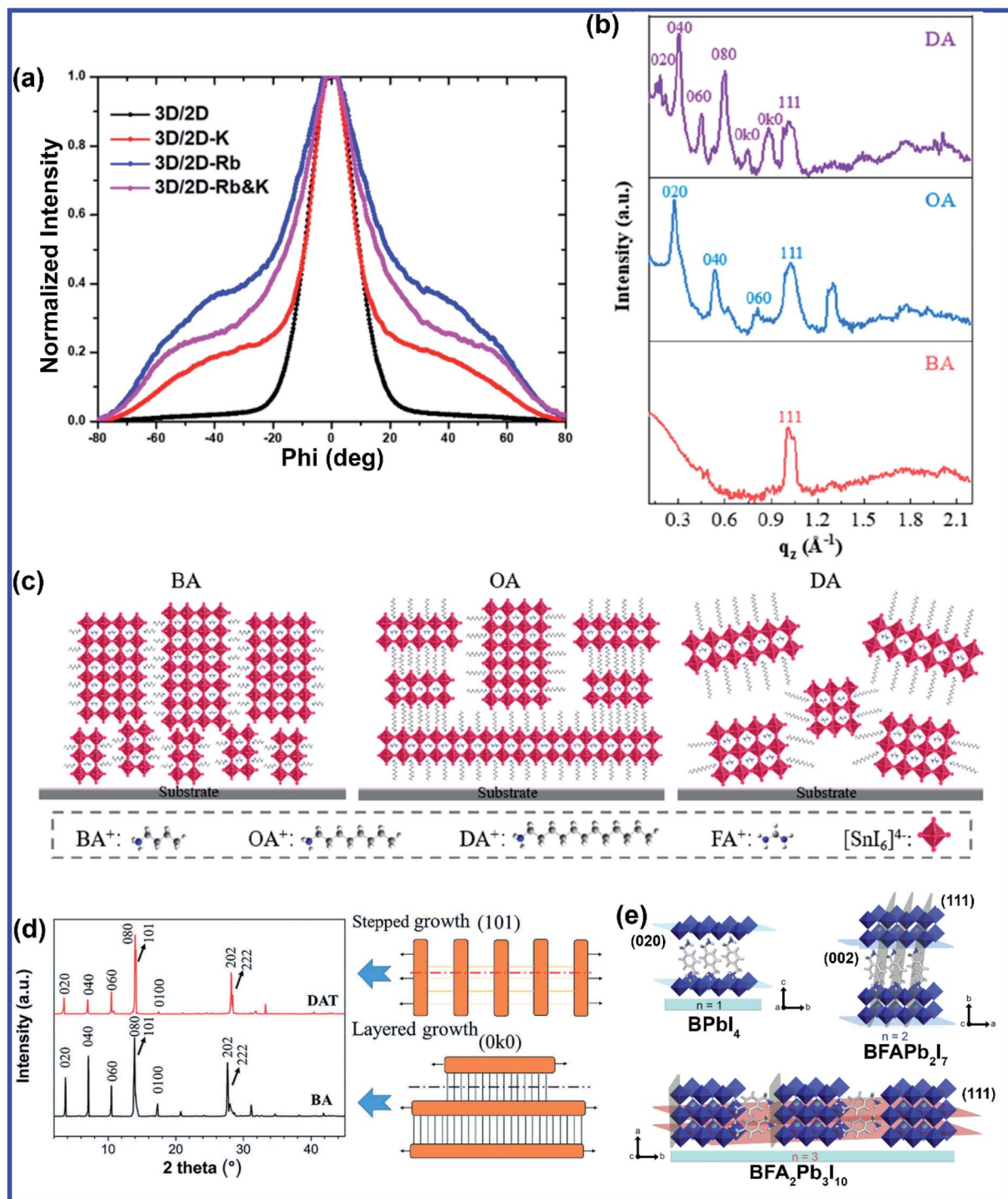
Fig. 4 (a) Integrated GIWAX patterns azimuthally over the ring at q = 0.33 \text{ \AA}^{-1} , corresponding to the (020) plane for alkali cation-doped (5% Rb + , 5% K + , and 5% Rb ++ + 5% K + ) 3D/2D perovskite. Reprinted with permission from ref. 54. Copyright 2020, American Chemical Society. (b) Comparison of GIWAX intensity profiles along the q_z axis and (c) schematic illustration of the crystal orientation of 2D perovskite films based on BA, OA and DA. Reprinted with permission from ref. 55. Copyright 2020, American Chemical Society. (d) Comparison of the XRD patterns of DAT and BA-based perovskites along with the schematic diagram of the proposed crystal growth mechanism for the 2D halide perovskite between BA and DAT. Reprinted with permission from ref. 56 with permission from the Royal Society of Chemistry. (e) Schematic representation of the crystal structure packing of the films with different \text{BFA}_{n-1}\text{Pb}_n\text{I}_{3n+1} perovskite compositions ( n = 1, 2 and 3 ). Reprinted with permission from ref. 60. Copyright 2019, American Chemical Society.
