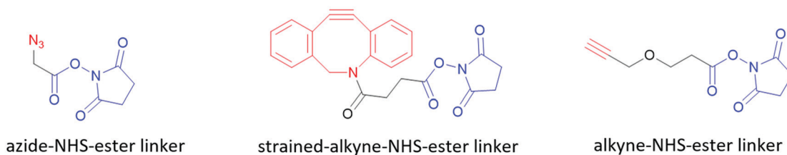
Fig. 10 Examples of commercially available non-natural nucleotides, non-natural amino acids and bioconjugation linkers functionalized with click chemistry handles. The click chemistry handles are highlighted red, the structural analogs of natural nucleotides and amino acids are highlighted green, and the handles attaching to amino groups (as discussed in Section 3.3.2) are highlighted blue.
