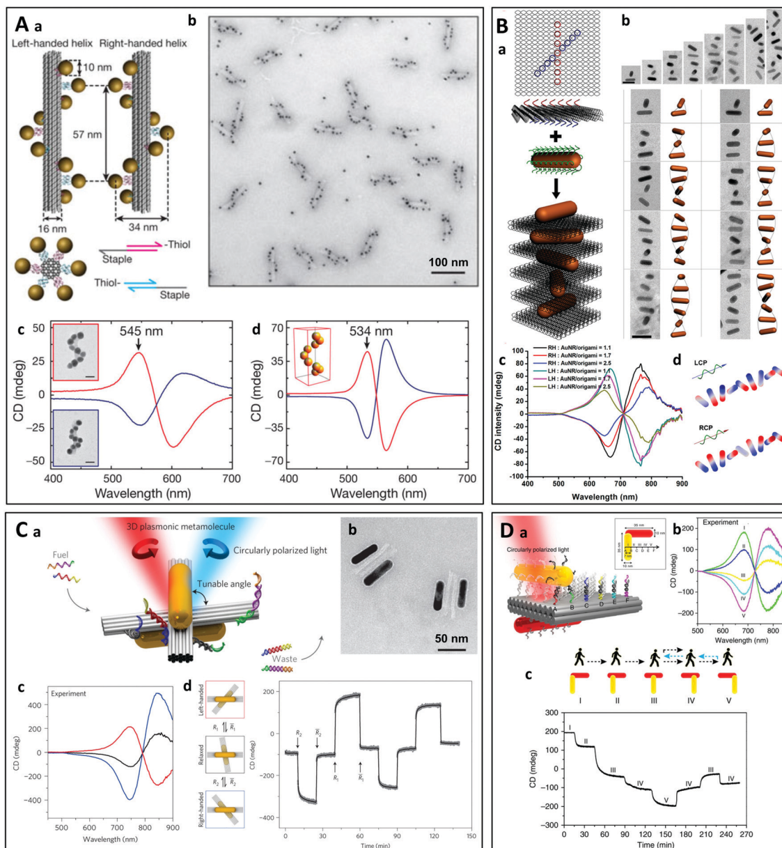
Fig. 8 (A) Schematic representation of left-handed and right-handed assembled on DNA bundles. (b) TEM image of assembled left-handed gold nanohelices. (c) and (d) Measured (c) and modeled (d) CD spectra of left-handed (red lines) and right-handed (blue lines) helices that are made from 16 nm gold nanoparticles. 126 Copyright 2012 Springer Nature. (B) (a) Schematic representation of the self-assembly of right-handed AuNR helices using a DNA origami. (b) Cryo-TEM images of the assembled AuNR helices containing varying numbers of AuNRs and the corresponding reconstructed models. (c) CD spectra of right-handed and left-handed helices containing varying number of AuNRs. (d) Calculated surface charge distribution profile of a right-handed helix upon induced by the illumination with LCP and RCP light. 163 Copyright 2015 American Chemical Society. (C) (a) Schematic representation of a gold nanorod dimer attached to two DNA bundles at a tunable angle. The CD of the structure can be modulated by adding specific DNA strands to change the angle between the two nanorods. (b) TEM images of the plasmonic metamolecules in the right-handed state. (c) CD spectra measured in the left-handed (red line), relaxed (black line) and right-handed (blue line) states. (d) The plasmonic metamolecules can be driven to either the left- or right-handed state by adding specific DNA strands ( R_1 and R_2 ). The CD signal was monitored over time at a fixed wavelength of 725 nm. 177 Copyright 2014 Springer Nature. (D) (a) Schematic of the plasmonic walker. Two gold nanorods (AuNRs) are assembled perpendicularly to one another on a double-layer DNA origami template, and the walking track comprises six rows of footholds (A–F) to define five walking stations (I–V). (b) Measured CD spectra at different stations. (c) Directional (forward and reverse) nanoscale “walking” of a nanorod on a DNA sheet leads to a change in the CD of the nanorod dimer. 178 Reproduced under the terms and conditions of the CC-BY license.
