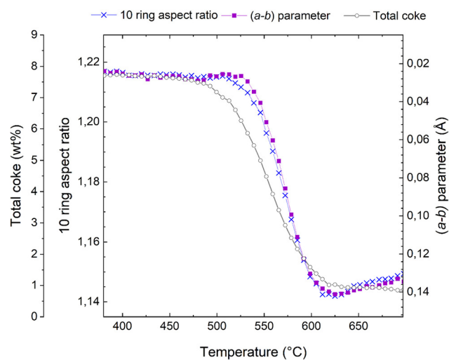
Fig. 4 Total coke content from dummy atom occupancies (connected grey open circles), evolution of the (a - b) parameter (connected purple squares, note that the scale is inverted relative to Fig. 2), and 10 ring aspect ratio (connected blue crosses) during the course of regeneration of the H-ZSM-5 catalyst.
