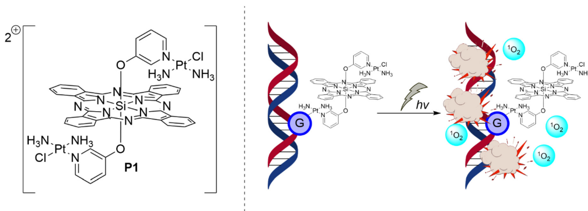
Fig. 6 Schematic PDT mechanism for Pc–platin conjugate P1 , where anchoring to DNA leads to highly effective damage by singlet oxygen formed upon photoirradiation of the Pc photosensitizer once coordinated to the DNA strand(s).
