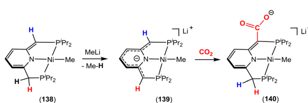
Scheme 42 Double deprotonation of a Ni–PNP pincer complex and further reactivity with CO 2 .
