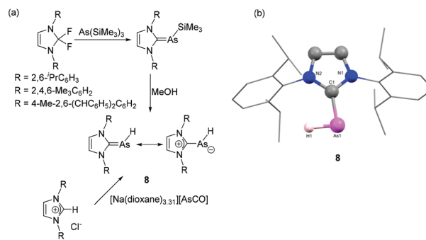
Fig. 4 (a) Synthesis of NHC-arsinidene 8 starting from [AsCO] – and As(TMS) 3 ; (b) solid-state structure of 8 .
