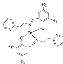
Scheme 2 Structures of the homoleptic Zn(II) complexes 1 – 6 .
