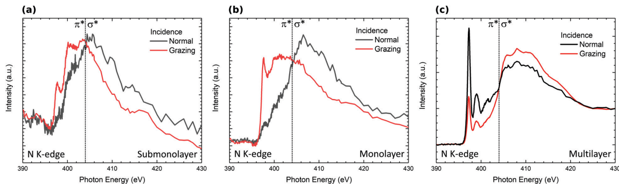
Fig. 5 Nitrogen K -edge NEXAFS spectra measured at normal ( E_{\parallel} substrate) and grazing ( E_{\perp} substrate) incidence for different H 2 Pc coverages: (a) submonolayer, (b) monolayer, and (c) multilayer coverages. Sharp features below 404 eV correspond to 1s \rightarrow \pi^* transitions and a broad feature above 404 eV corresponds to 1s \rightarrow \sigma^* transitions.
