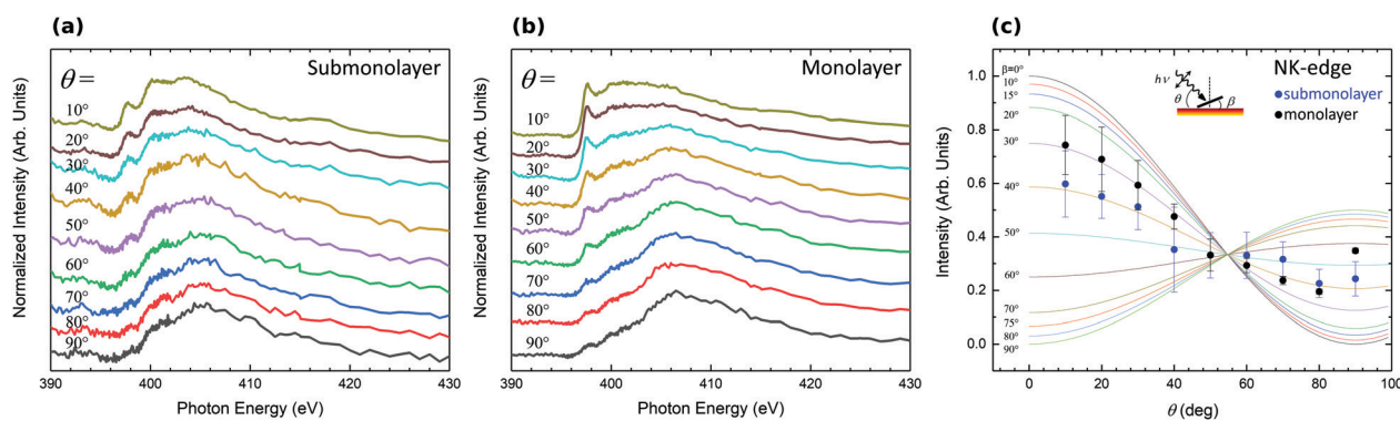
Fig. 6 Angular-dependent N K -edge NEXAFS spectra for submonolayer (1/6th) (a) and monolayer (b) H 2 Pc molecules on the 6H-SiC(0001)-(3 × 3) surface. (c) Intensities of the main 1s \rightarrow \pi^* resonance against \theta for submonolayer (blue circle) and monolayer (black circle) H 2 Pc coverages. The solid lines represent the theoretical angular variation of 1s \rightarrow \pi^* resonances calculated for various molecular tilt angles. The inset shows the schematic diagram of the measured geometry.
