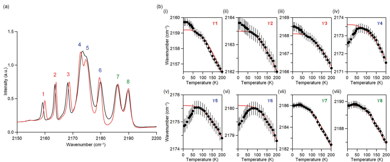
Fig. 3 Temperature dependence of the IR spectrum of MnW. (a) IR spectrum at 5 K (red) and 60 K (black). (b) IR peak frequency due to the CN stretching mode, \nu_i ( i = 1 – 8 ), vs. temperature plots. Red line indicates the peak position obtained by fitting the theoretical equation of thermal expansion 61 due to anharmonic phonons without magnetic ordering. Error bars indicate the resolution of the apparatus.
