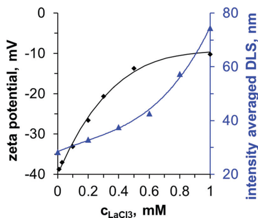
Fig. 3 Colloidal stability of Ludox-TM in dependence of the \text{La}^{3+} concentration (pH 9). The corresponding DLS polydispersity index range from 0.18 (0 mM)–0.48 (1 mM), see ESI. ^\dagger
