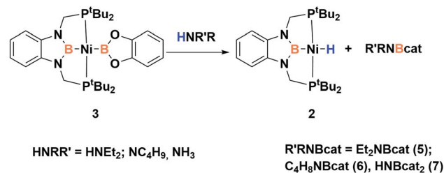
Scheme 5 Reactivity of 3 with amines and ammonia.
