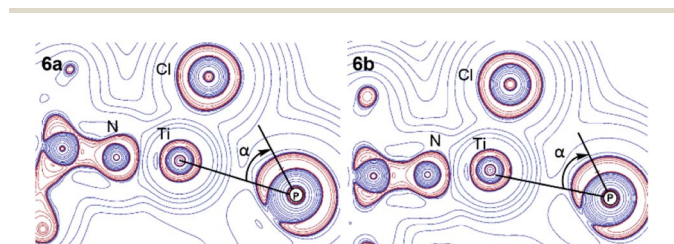
Fig. 8 Contour map of \nabla^2\rho in the \text{P}_c\text{--Ti--Cl} plane for 6a and 6b (red lines indicate charge concentration and blue lines indicate charge depletion).
