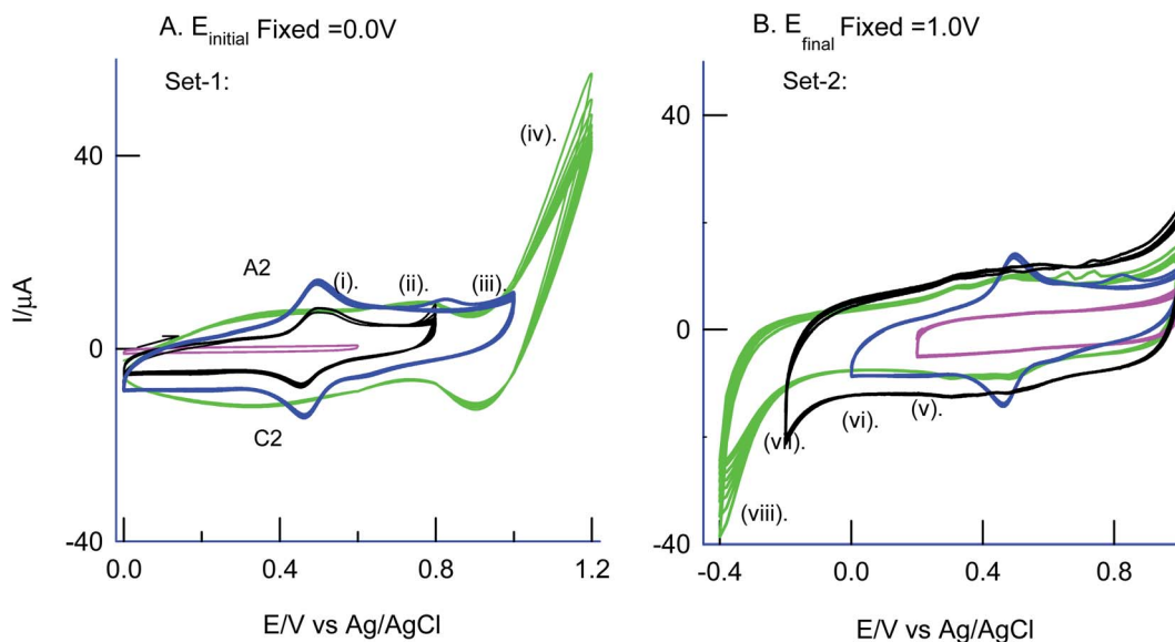
Fig. 5 Effect of bias potential on CV response of GCE/Nf-MWCNT (freshly prepared electrodes) with 50 mM PhOCH 3 + 6 mM H 2 O 2 in pH 2 KCl-HCl buffer at \nu = 50 \text{ mV s}^{-1} (A) CV experiments with a fixed starting/initial potential of 0.0 V and varying switching final potential of (i) 0.6 V, (ii) 0.8 V, (iii) 1.0 V and (iv) 1.2 V vs. Ag/AgCl. (B) CV experiments with a fixed final potential of 1.0 V and varying initial potentials from (v) -0.4 V, (vi) -0.2 V, (vii) 0.0 V and (viii) 0.2 V vs. Ag/AgCl.
