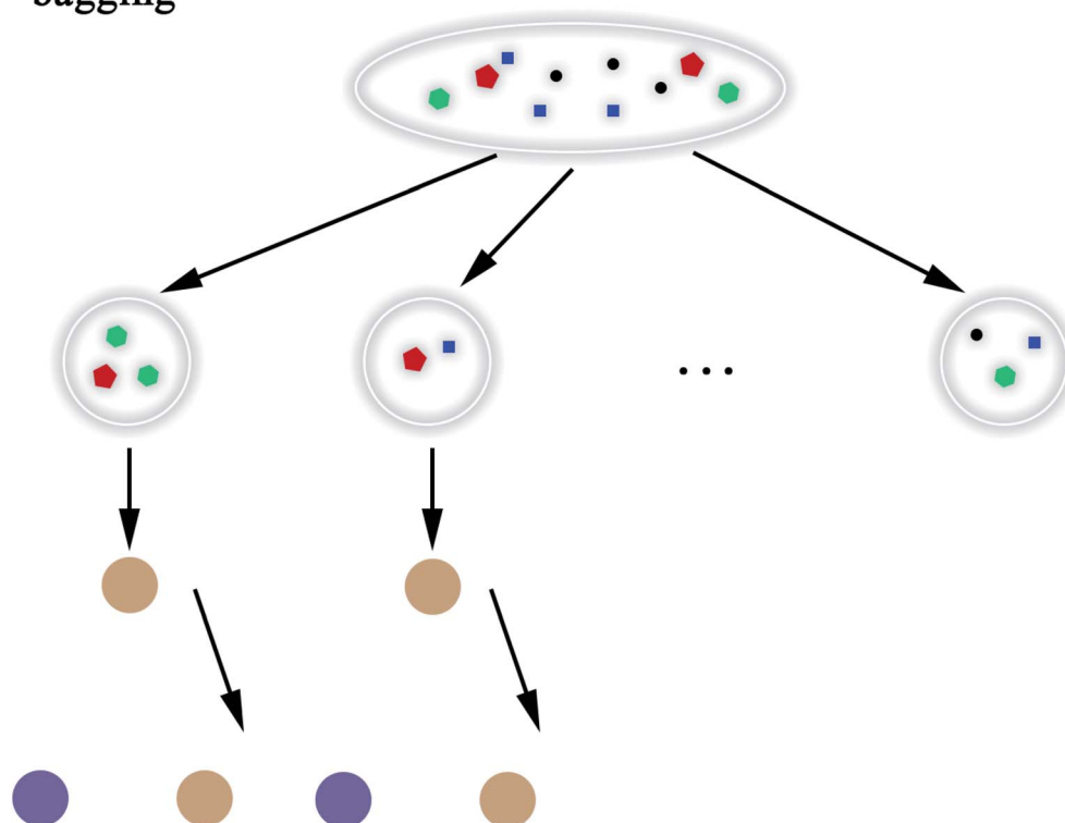
Fig. 9 Schematic diagram of bagging.
