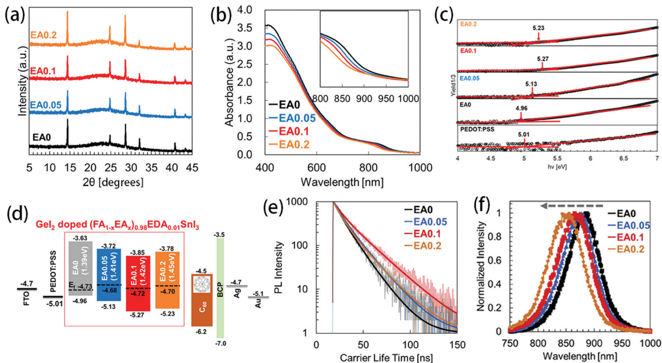
Fig. 6 (a) XRD patterns of GeI 2 doped (FA 1-x EA x ) 0.98 EDA 0.01 SI 3 perovskite films with different amount of EA incorporated. (b) UV-Vis measurement of GeI 2 doped (FA 1-x EA x ) 0.98 EDA 0.01 SI 3 perovskite films with different amount of EA incorporated. (c) The PYS measurement of perovskite films with different EA amount. (d) The schematic illumination of band alignment for the PSC with various EA amount. (e) Normalized PL spectra and (f) TRPL spectra of perovskite films with various EA amount. 14 Copyright 2020, Elsevier.
