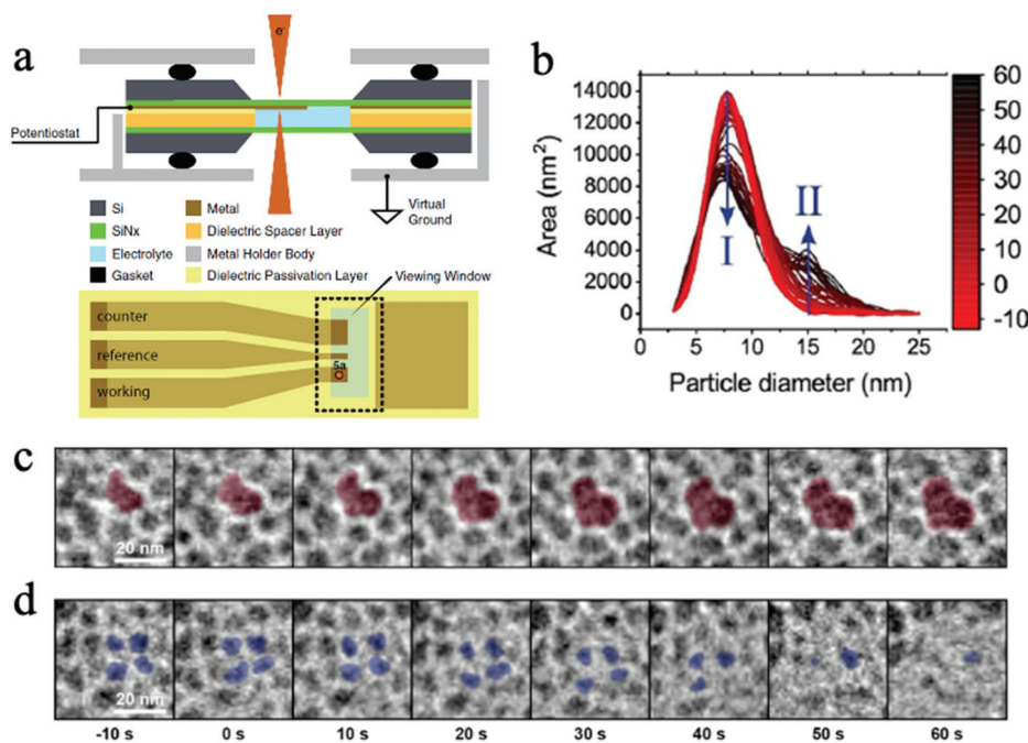
Fig. 6 (a) The schematic of a micro electrochemical cell for in situ TEM. Copyright 2017, IOP Publishing, Inc.; (b) the change in primary (I) and secondary (II) particle sizes as experiment progresses; (c) the growth of secondary particles, and (d) the shrinkage of primary particles. Copyright 2020, John Wiley and Sons. All panels reproduced with permission. 152,154
