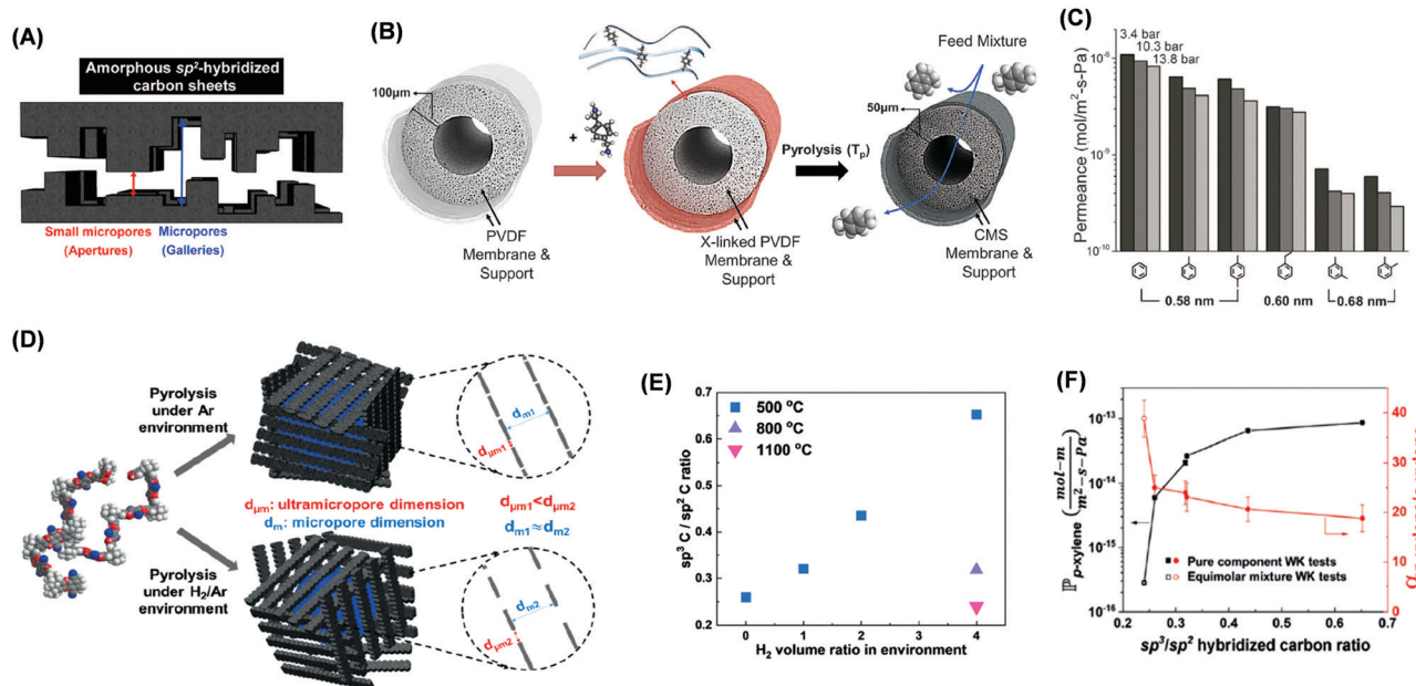
Fig. 11 (A) Schematic representation of bimodal CMS slit-like structure consisting of ultramicropores and micropores. (B) Cross-linking of PVDF hollow fibers using p -xylenediamine followed by carbonization to form CMS. (C) The permeance of aromatic hydrocarbons through C-PVDF CMS as a function of their molecular size at 3.4, 10.3, and 13.8 bar. 4 Copyright 2020, Science. (D) Increase of ultramicropore sizes by H 2 in the carbonization atmosphere. (E) Effect of the H 2 content in the pyrolysis atmosphere on the SP 3 /SP 2 carbon ratio in CMS. (F) p -xylene/ o -xylene separation properties as a function of SP 3 /SP 2 carbon ratio. 49 1 mol m -2 s -1 Pa -1 = 3.6 × 10 5 / M W /ρ (LMH per bar m -1 ). Copyright 2019, Wiley-VCH.
