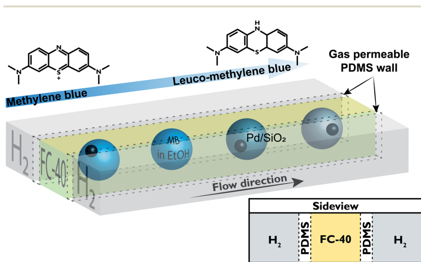
Fig. 1 Schematic representation of a polydimethylsiloxane (PDMS) microreactor with three parallel channels separated by 50 \mu\text{m} thick walls. H_2 can diffuse through the walls and hydrogenate methylene blue (MB) to leuco-MB in the presence of Pd/SiO 2 particles in ethanol droplets.
