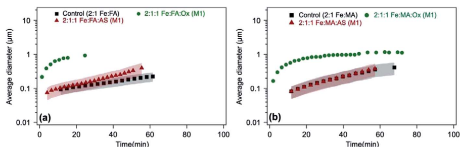
Fig. 19 Effect of adding oxalate (Ox) and ammonium sulfate (AS) on particle size from time-dependent DLS measurements during the dark aqueous phase reaction of (a) fumarate ( 50 \mu M , FA) and (b) muconate ( 25 \mu M , MA). This molar ratio results in the maximum product mass per data shown in Fig. 1. ‘M1’ stands for method 1, where organic reagents were mixed first with AS or Ox, then the reaction time started when Fe was added. ‘M2’ stands for method 2, where AS or Ox were reacted first with Fe for 2 h, then the reaction time started when the organic reagent was added. The shaded areas represent the standard deviation of three trials. Unshaded data represent the average of two trials, with a standard deviation the size of the marker width (15%). Reproduced from ref. 68 with permission from the American Chemical Society, © 2021.
