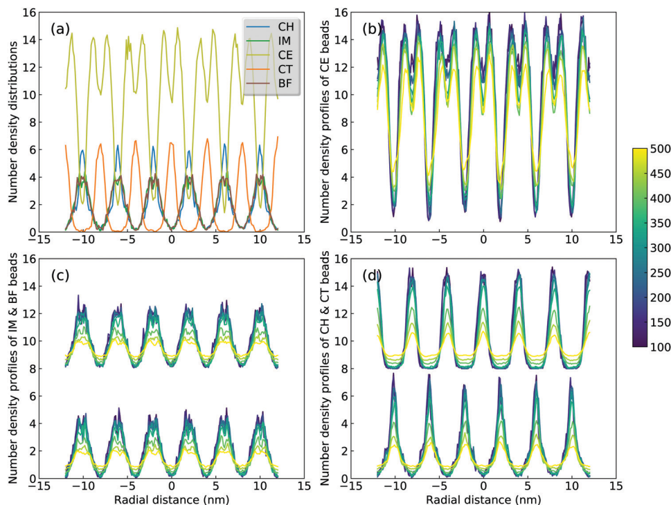
Fig. 11 Number density distributions of (a) CG beads in [C_2C_{12}IM][BF_4] ILs along z -axis at 300 K, and of (b) CE, (c) IM and BF, and (d) CH and CT beads at different temperatures. The density profiles for BF and CT beads are vertically shifted by eight units for clarity.
