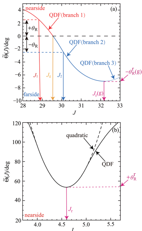
Fig. 5 Plots for the 000 \rightarrow 000 transition of Fig. 4(a) at E_{\text{trans}} = 1.35 eV giving the notations used in the SC glory and rainbow theories for all four transitions. (a) \hat{\theta}(J)/\text{deg} versus J close to J = J_g for the range J = 28 to J = 33 . The three branches of the QDF used in the SC analysis are indicated: branch 1 (nearside, red solid curve), branch 2 (farside, blue solid curve) and branch 3 (farside, blue dotted curve). The values of \hat{\theta}(J)/\text{deg} at the angles +\theta_R and -\theta_R are indicated by a red dashed line (nearside) and a blue dashed line (farside) respectively. The corresponding values of the total angular momentum variable are denoted J_1 \equiv J_1(\theta_R) (red solid arrow) and J_2 \equiv J_2(\theta_R) (blue solid arrow) respectively. The orange arrow indicates J_g , which satisfies \hat{\theta}(J_g) = 0 . The pink solid arrow shows the rainbow total angular momentum variable, J_r , which is close to J_g . The corresponding rainbow value of \hat{\theta}(J)/\text{deg} is denoted -\theta_r^f(g) (pink dashed line). (b) \hat{\theta}(J)/\text{deg} versus J for the range, J = 3.7 to J = 5.7 . The pink solid arrow shows the rainbow total angular momentum variable, J_r . The corresponding nearside rainbow value of \hat{\theta}(J)/\text{deg} is denoted +\theta_r^f (pink dashed line). The black dashed curve shows the quadratic approximation to \hat{\theta}(J)/\text{deg} .
