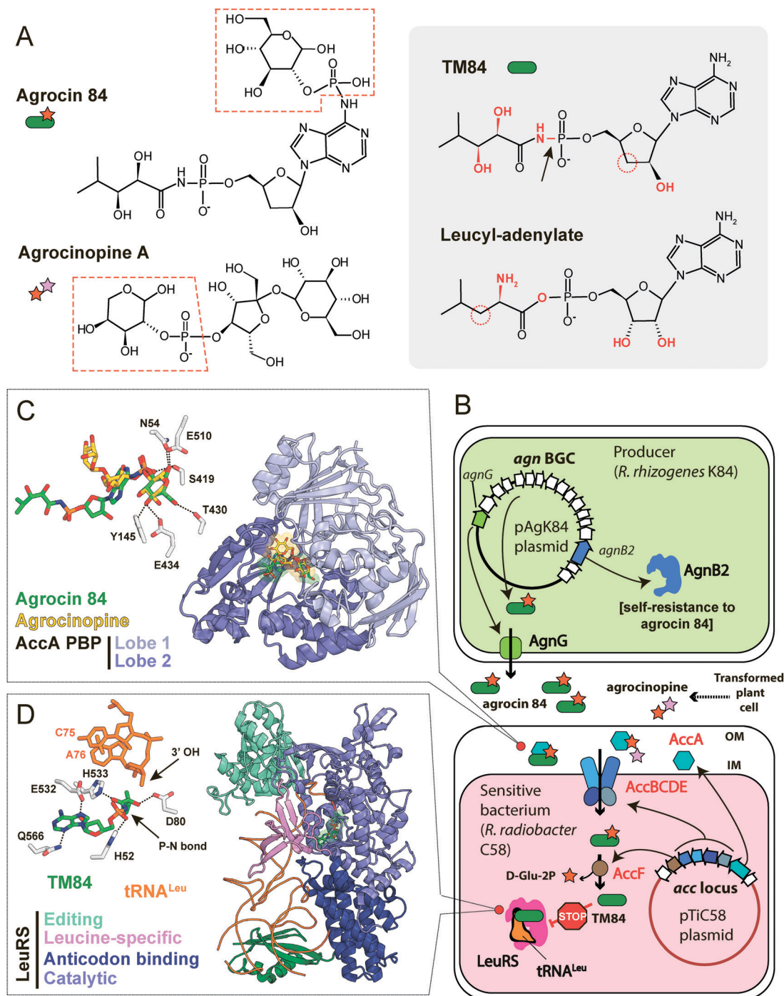
Fig. 8 (A) Chemical structures of agrocins 84, its toxic moiety (TM84), agrocinopine A and leucyl-adenylate. Pyranose-2-phosphate groups shared by agrocins 84 and agrocinopine A are highlighted with red dashed polygons. Groups of atoms that are different between TM84 and leucyl-adenylate are shown in red. The black arrow indicates a nonhydrolyzable P–N bond in TM84. (B) The scheme showing the biosynthesis, transport, and mode of action of agrocins 84. IM – inner membrane, OM – outer membrane, BGC – biosynthetic gene cluster, LeuRS – leucyl-tRNA synthetase. (C) The details of the interaction between agrocins 84/agrocinopine A with the periplasmic solute binding protein (PBP) AccA (PDB IDs: 4ZEC/4ZEB). 109 Agrocinopine is coloured gold, agrocins 84 is green. Amino acid residues interacting with D-glucopyranose-2-phosphate moiety of agrocins are shown in the left corner. Hydrogen bonds are shown as black dashed lines. (D) The crystal structure of the ternary complex of LeuRS, TM84 and tRNA Leu (PDB ID: 3ZGZ). 118 Selected amino acid residues involved in the binding of TM84 in the active site of LeuRS are shown in the left corner together with the two 3'-terminal nucleotides of the tRNA Leu acceptor stem. TM84 is green, tRNA Leu is orange.
