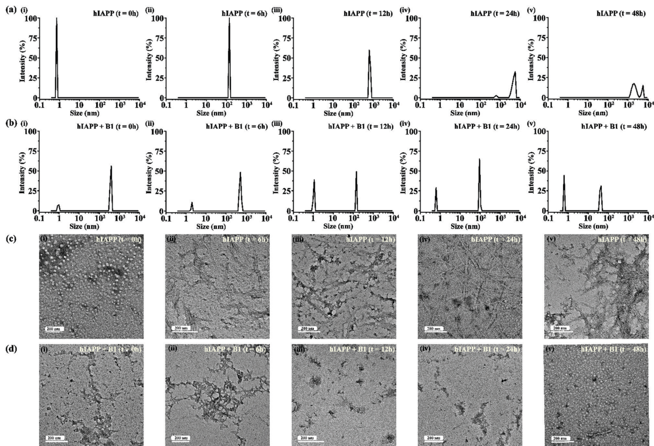
Fig. 5 DLS results showing the size distribution of hIAPP (40 \mu\text{M} ) alone (a) and in presence of 2-fold molar ratio of B1 (b) at 0 h (i), 6 h (ii), 12 h (iii), 24 h (iv) and 48 h (v) of incubation respectively. TEM images showing morphological change of hIAPP (40 \mu\text{M} ) alone (c) and in presence of 2-fold molar ratio of B1 (d) at 0 h (i), 6 h (ii), 12 h (iii), 24 h (iv) and 48 h (v) of incubation respectively. The scale bar in the TEM images indicate 200 nm.
