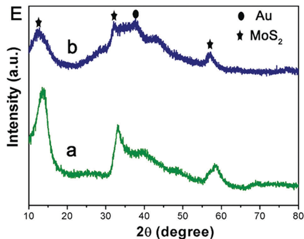
Fig. 2 SEM and TEM images of \text{PPy}@MoS_2 (A and B) and \text{PPy}@MoS_2 @Au (C and D) and (E) XRD patterns of \text{PPy}@MoS_2 (a) and \text{PPy}@MoS_2 @Au (b). Scale bars: 1 \mu\text{m} in (A) and 500 nm in (B–D).
