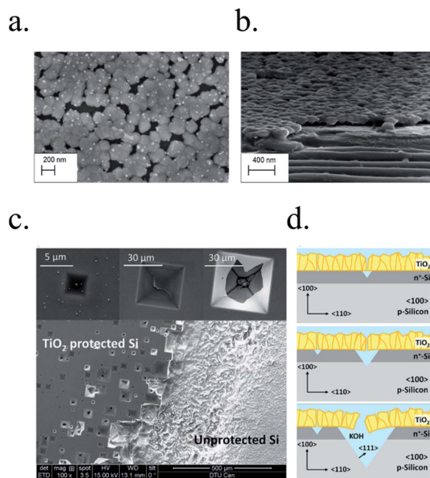
Fig. 15 (a) Top and (b) cross section SEM images of an almost-crystalline \text{TiO}_2 layer after a stability test in 0.5 \text{ M H}_2\text{SO}_4 , wherein dissolution of the amorphous region between crystals can be seen. Reprinted with permission from ( ACS Appl. Mater. Interfaces , 2017, 9 , 17932–17941). Copyright (2017) American Chemical Society. 238 (c) SEM images of a \langle 100 \rangle Si \text{TiO}_2 -protected and unprotected after immersion in 1 \text{ M KOH} for 3 days. (d) Schematics of the anisotropic etching process forming characteristic inverted pyramids. Reprinted with permission from ( Sol. Energy Mater. Sol. Cells , 2016, 144 , 758–765). Copyright (2016) Elsevier. 145
