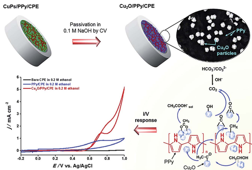
Fig. 14 The preparation of Cu 2 O/PPy/CPE for ethanol electrocatalytic oxidation. Reproduced with permission from ref. 128. Copyright 2020 Elsevier.
