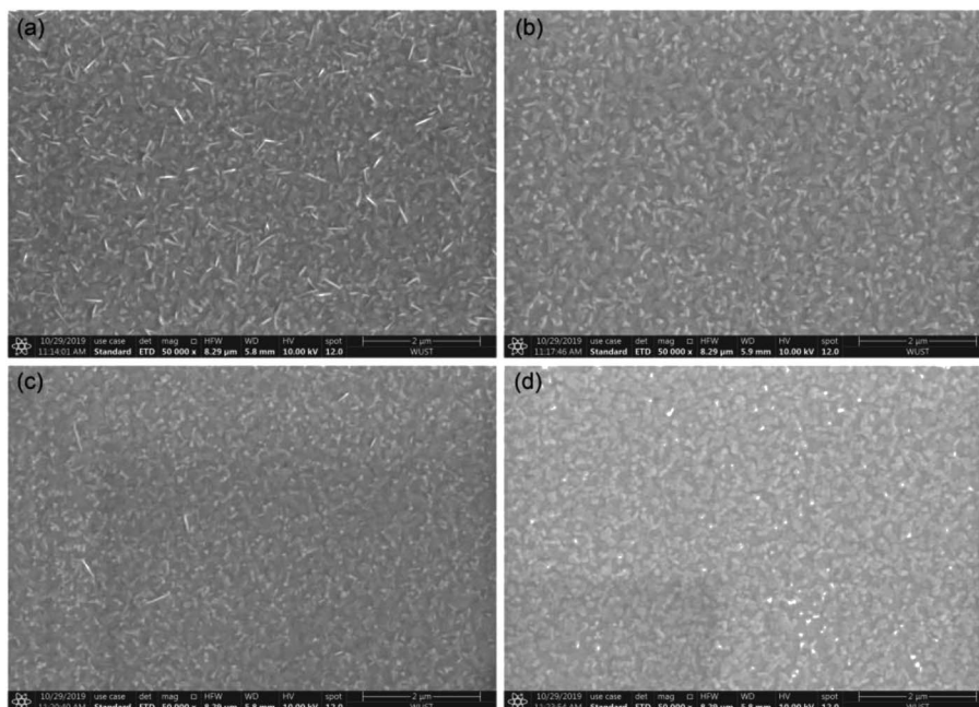
Fig. 4 SEM images of the \text{CH}_3\text{NH}_3\text{PbBr}_3 films on the GO-doped composite films with different GO concentration of (a) 1 : 0, (b) 1 : 0.1, (c) 1 : 0.3, (d) 1 : 0.5.
