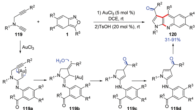
Scheme 44 Gold-catalysed annulation of terminal N -propargyl ynamides and anthranils.
