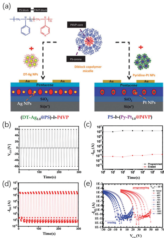
Fig. 9 (a) Schematic illustration of the device structures of pentacene based OFET memory devices and the distributional positions of DT-Ag and Py-Pt NPs within them. Inset: The chemical structure of the PS- b -P4VP copolymer. Reproduced with permission. 57 Copyright 2012, Royal Society of Chemistry. (b) P/E bias pulses of -60 V were repeatedly applied to the bottom-gate electrode for 5 s (programming: V_G = 60 V and V_D = -10 V and erasing: V_G = -60 V and V_D = -10 V). (c) The retention time for the 27 nm thick PS 56k - b -P4VP 8k memory device in the programmed/erased states under ambient conditions at room temperature. The dotted line is the extrapolation of the measurement data, which is used to determine the long-term reliability of the storage devices. (d) The 27 nm thick PS 56k - b -P4VP 8k thin film is used to realize the reversible switching of the on-off state of the polymer electret OFET memory. (e) Shifts in transfer characteristics at V_D = -10 V for the 27 nm thick PS 56k - b -P4VP 8k polymer electret OFET memory device, where V_G = 60, 70, 80, 90, and 100 V and V_G = -60, -70, -80, -90, and -100 V were applied for 3 s for programming and erasing, respectively. Reproduced with permission. 56 Copyright 2013, Royal Society of Chemistry.
