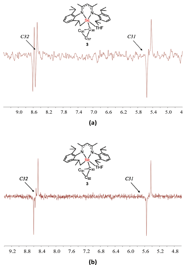
Fig. 5 ^{13}\text{C} - ^{13}\text{C} INADEQUATE spectra of 3 , optimized for J = 3 Hz (a) and J = 15 Hz (b), respectively.
