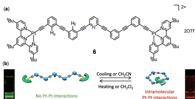
Fig. 5 (a) Molecular structure of Pt(II) complex 6 . (b) Schematic diagram showing the reversible helix–coil molecular configuration transformation regulated by solvents and temperature. Reprinted with permission from ref. 93. Copyright 2019 American Chemical Society.
