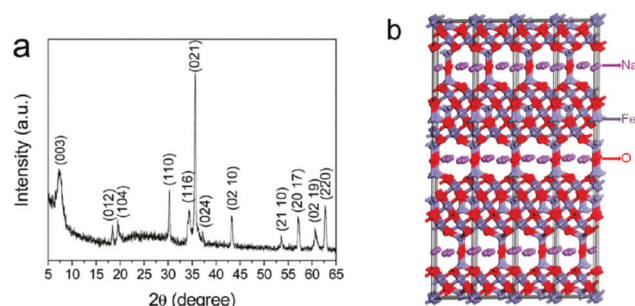
Fig. 17 (a) XRD pattern of sodium iron oxide nanosheets synthesised under microwave irradiation at 180 °C for 5 min. (b) Crystal structure of Na_{2.4}Fe_{10.99}O_{16.03} viewed perpendicular to the c axis. The pink, red, and grey spheres correspond to Na, O, and Fe atoms, respectively. Reproduced with permission from Wu et al. 328
