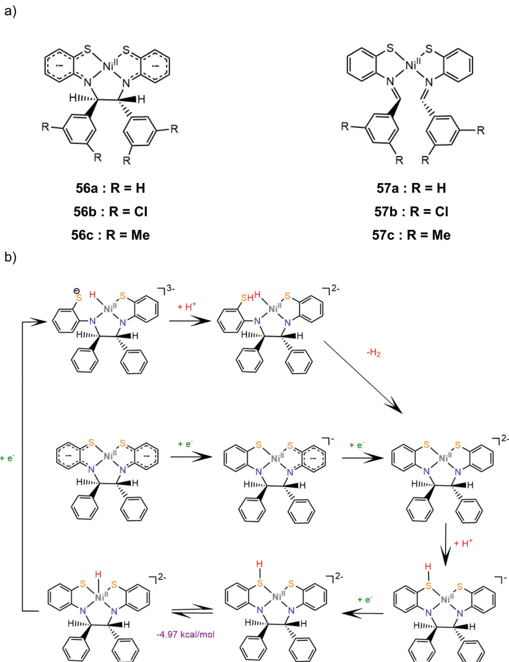
Scheme 25 (a) Molecular structures of complexes carrying Schiff based ligands. (b) Proposed mechanism catalysed by complex 56a.
