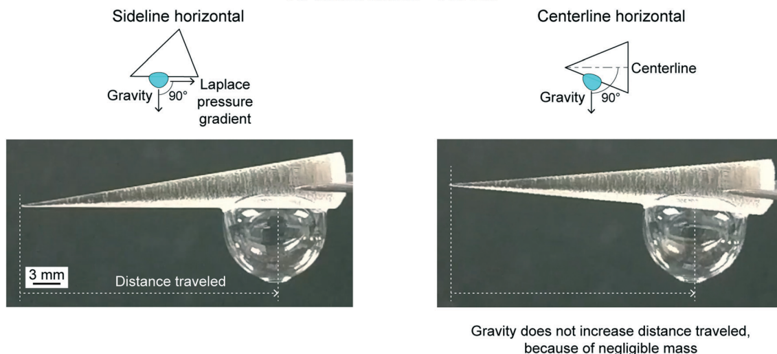
Fig. 12 Effect of cone orientation on air bubble movement with optical images of 500 \text{ mm}^3 volume air bubbles at equilibrium at two cone orientations (adapted from ref. 18).
