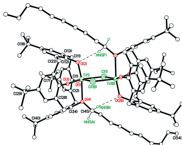
Fig. 2 Molecular structure of \{[\text{Ti}(\text{L}(\text{O})_3(\text{OR})_2)(\mu\text{-Cl})_2] \cdot 6\text{MeCN}\} ( R = n\text{-decyl} (4·6MeCN)) (most H atoms and solvent molecules are omitted for clarity). Selected bond lengths (Å) and angles ( ^\circ ): Ti(1)–Cl(1) 2.4454(12), Ti(1)–Cl(1B) 2.5257(10), Ti(1)–O(1) 1.794(2), Ti(1)–O(2) 1.825(3), Ti(1)–O(3) 1.792(3), Ti(1)–O(4) 2.390(3); Ti(1)–O(1)–C(1) 161.5(2), Ti(1)–O(2)–C(12) 121.9(2), Ti(1)–O(3)–C(23) 158.1(3), Ti(1)–O(4)–C(34) 115.0(2), Cl(1)–Ti(1)–Cl(1B) 77.04(4).
