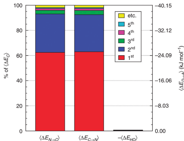
Fig. 2 Average contributions of the five strongest acceptor ( \Delta E_{\text{N}\rightarrow\text{C}} ) and donor ( \Delta E_{\text{C}\rightarrow\text{N}} ) interactions. The right-most column shows that higher-order delocalization does not significantly contribute to the overall binding (see also shaded areas in Fig. 5). Angular brackets within the axes labels denote averaging over all central water molecules and all AIMD snapshots. Reproduced from ref. 13.
