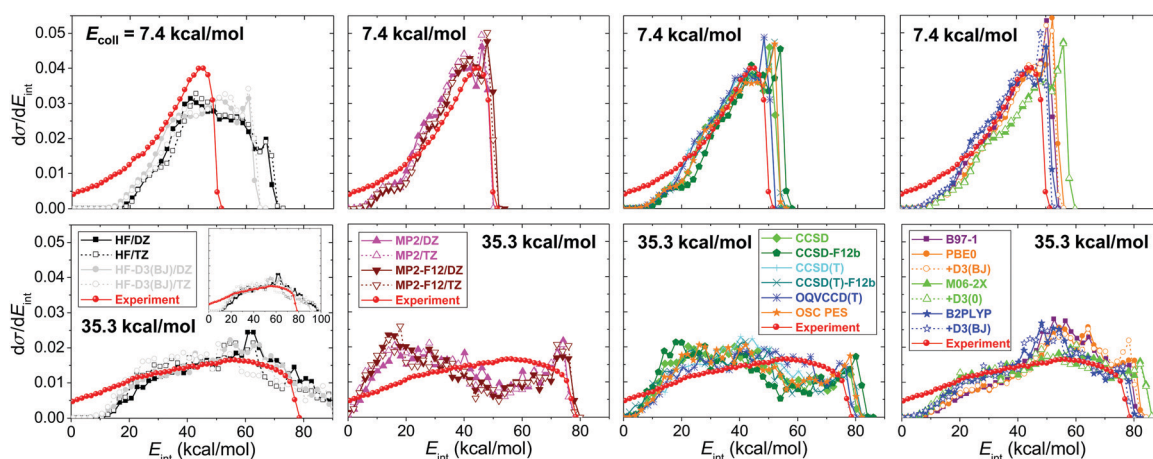
Fig. 12 Normalized product internal energy distributions for the F^- + CH_3I S_N2 reaction obtained on various ab initio - and DFT-based analytical PESs (see Fig. 11 for notations) at collision energies of 7.4 and 35.3 \text{ kcal mol}^{-1} . 71 The experimental data are taken from ref. 122.
