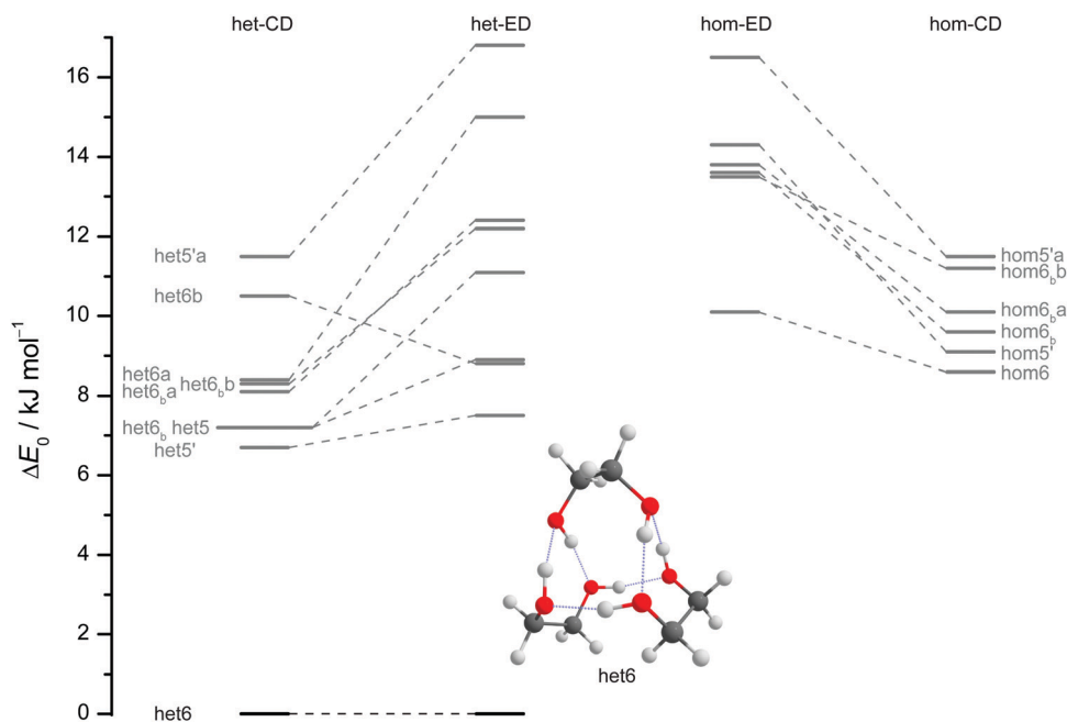
Fig. 8 ZPV-corrected relative energies of the lowest 15 trimer structures for ED (inner) and CD (outer) at B3LYP-D3/def2-TZVP level, distinguishing between heterochiral (left) and homochiral (right) pairings. Energy levels in grey were not considered for the interpretation of the experimental spectra. Dashed lines connect corresponding ED and CD structures and thus visualise the effect of the cyclohexyl substitution.
