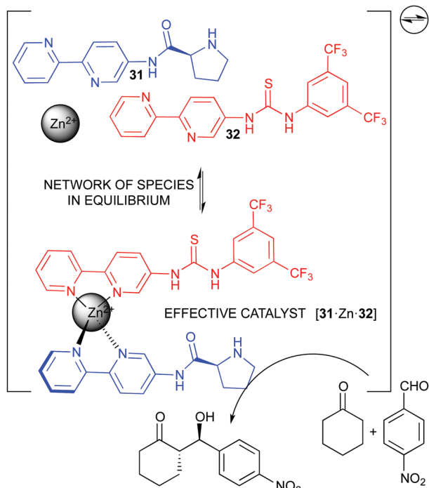
Fig. 17 Dynamic network of organocatalytic bipyridine ligands templated by Zn^{2+} .
