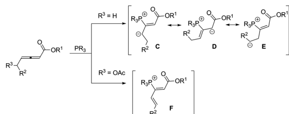
Scheme 1 The reactivity of allenoates in the presence of organophosphines.
